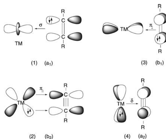
Scheme 2. Bonding orbital interactions between a transition-metal atom (TM) and an alkyne moiety ( \text{R}-\text{C}\equiv\text{C}-\text{R} ).
